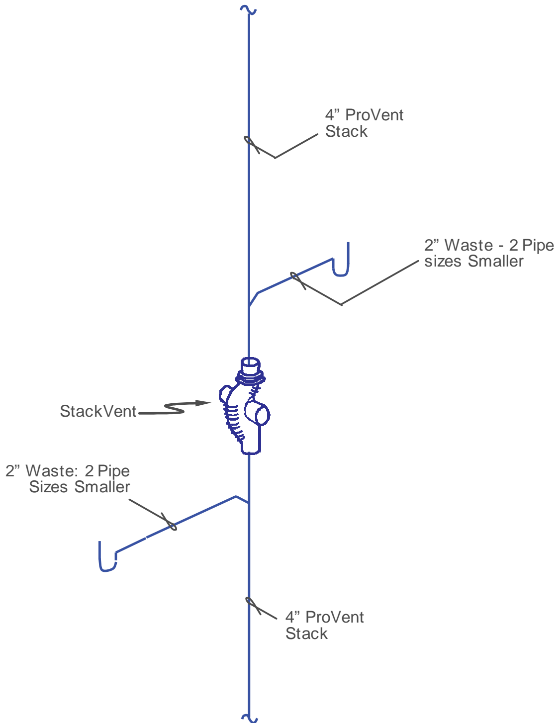
Drawing 1.3
