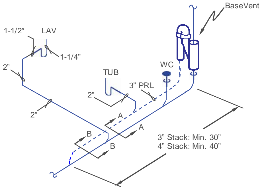
Drawing 33b
