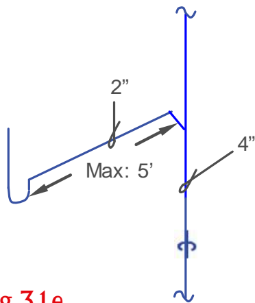
Drawing 31e
