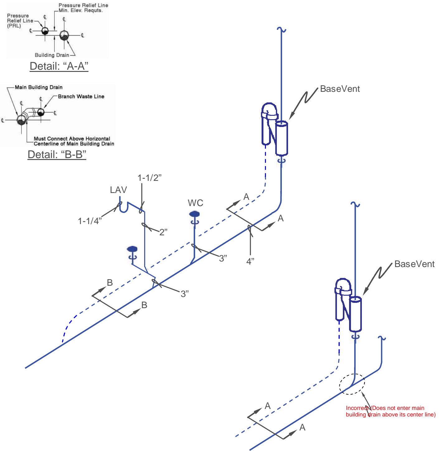
Drawing 2.4
