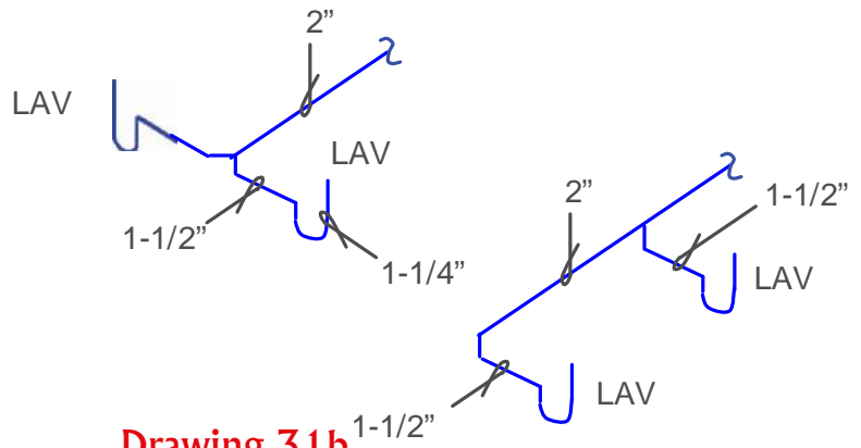
Drawing 31b
