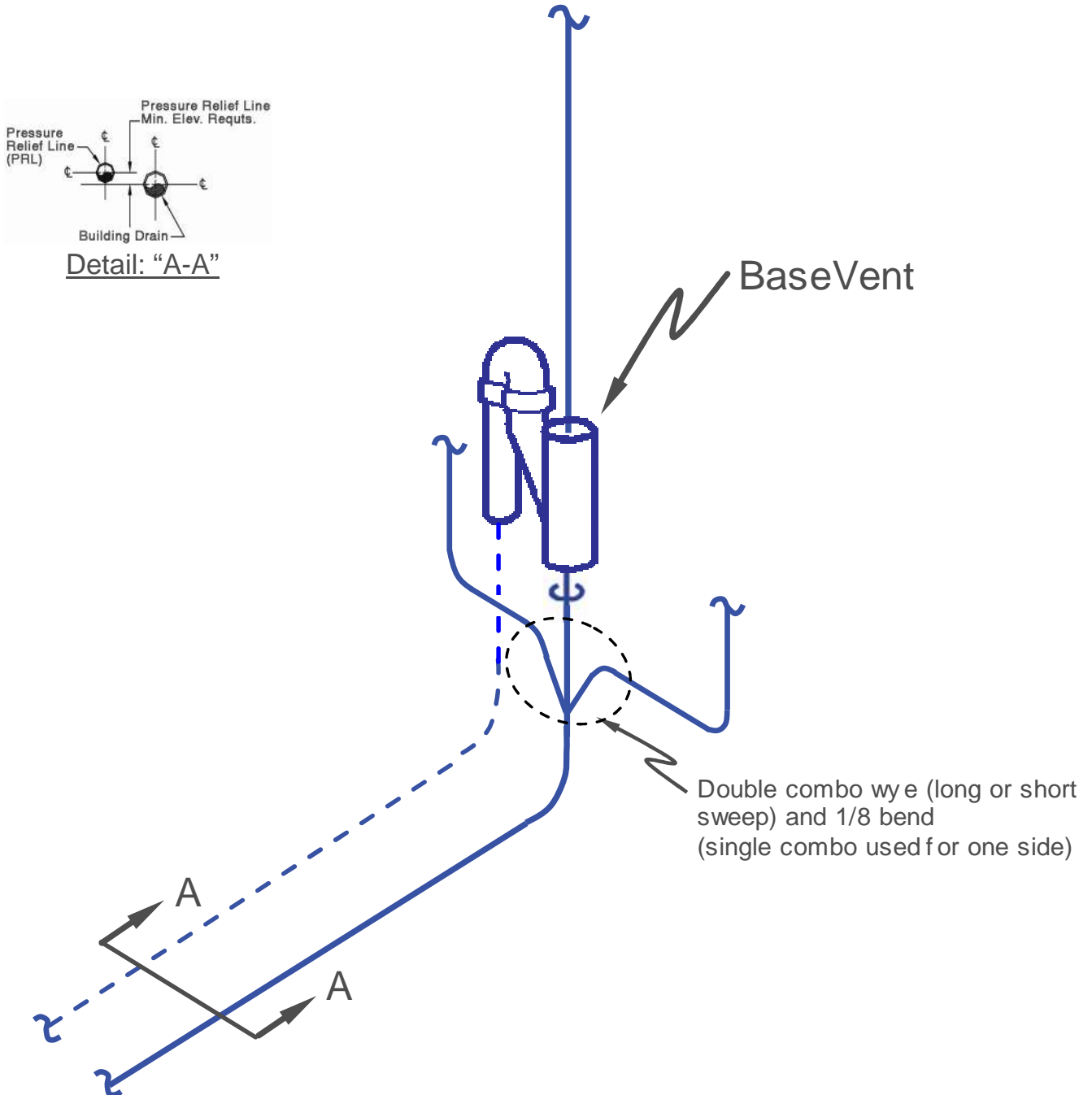
Drawing 2.6
