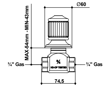
04500 Rubinetto incasso 1/2" 1/2" built-in tap 04498 Rubinetto incasso 3/4" 3/4" built-in tap
