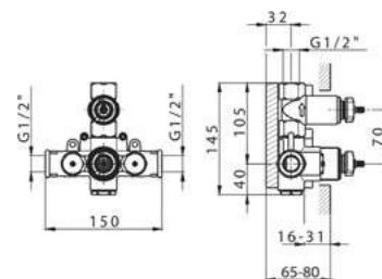
ZA 007301 Parte Incasso Termostatico Doccia Thermo Shower Concealed Part Partie Encastrée Thermo Douche
