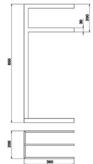
QU 090910 Porta Salviette Free-Standing Towel Rail Porte-Serviette
