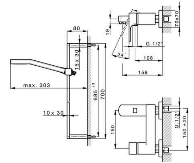
CU 00062 Completo Monocomando Vasca Bath/S. Mixer Set Ensemble Mitigeur Bain/D.
