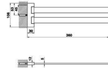
QU 090210 Porta Salviette Towel Rail Porte-Serviette
