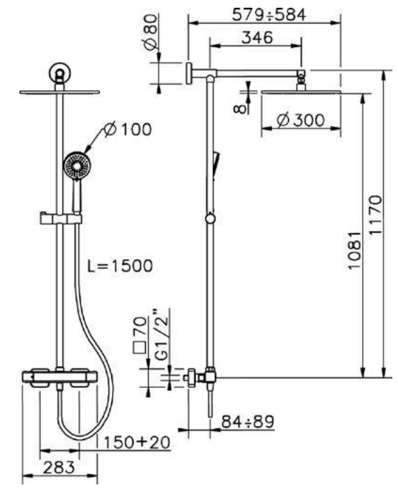
CU C78075 CombiDoccia Termostatico Thermo CombiShower CombiDouche Thermo
