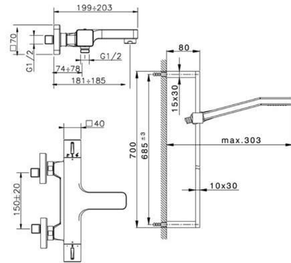
CU S21020 Completo Termostatico Vasca Thermo Bath/S. Set Ensemble Thermo Bain/D.
