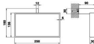
QU 090220 Porta Salviette Towel Rail Porte-Serviette
