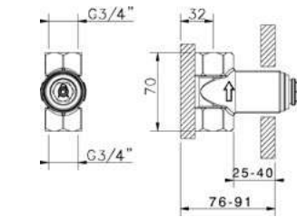
ZA 003330 Parte Incasso Rubinetto 3/4" 3/4" Stopvalve Concealed Part Partie Encastrée Robinet 3/4"
