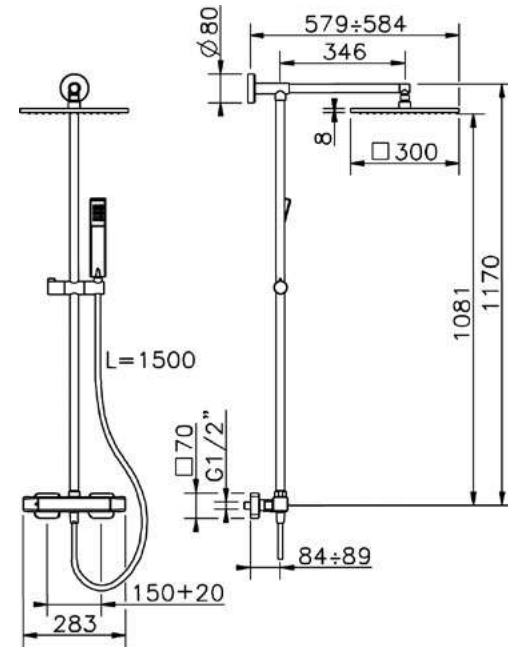
CU C78085 CombiDoccia Termostatico Thermo CombiShower CombiDouche Thermo
