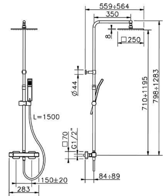
CU C8401C CombiDoccia Termostatico Thermo CombiShower CombiDouche Thermo
