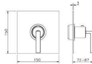
WA 007200 Parte Esterna Termostatico 3/4" 3/4" Thermo Exposed Part Partie Décor Thermo 3/4"
