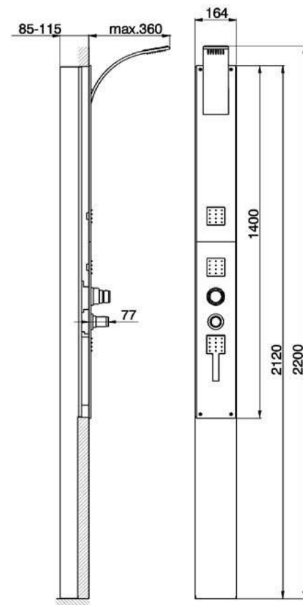
WA 00500 CombiDoccia Termostatico Thermo CombiShower CombiDouche Thermo
