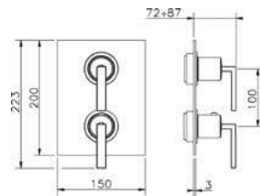
WA 009300 Parte Esterna Termostatico Doccia Thermo Shower Exposed Part Partie Décor Thermo Douche
