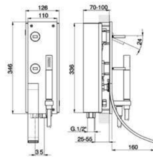
WA 001100 Completo Monocomando Vasca Bath Mixer Set Ensemble Mitigeur Bain/D.
